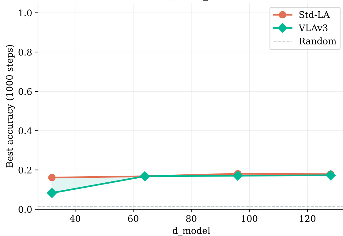
MQAR Accuracy vs d_model (8 pairs)
