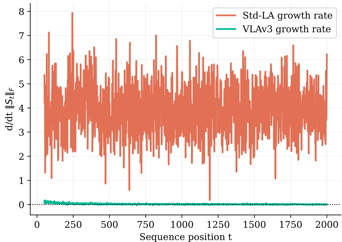
(b) Rate of State Norm Growth
