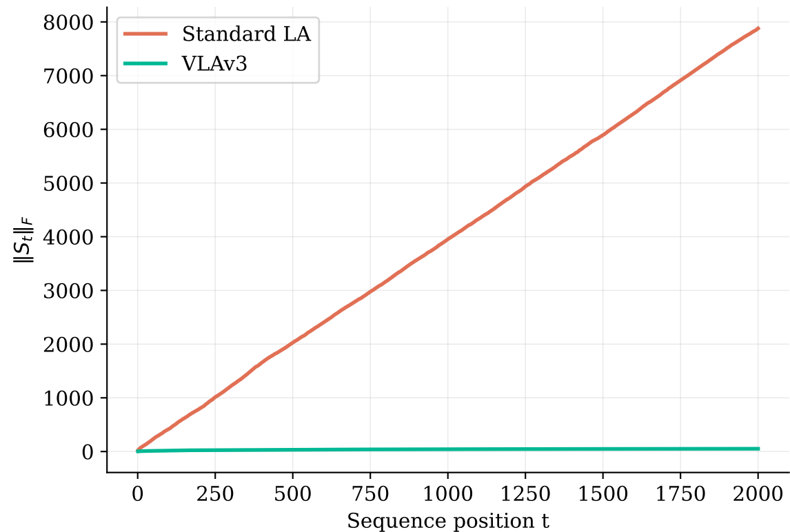
(a) KV State Norm Growth
