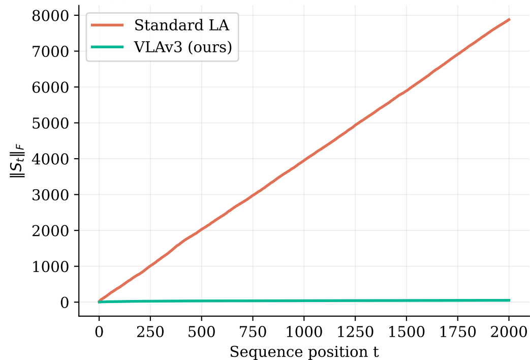
(a) KV State Norm ( 152\times lower at T=2000 )
