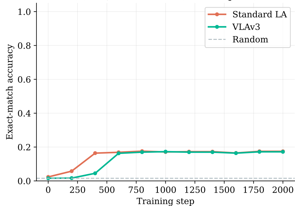
(b) MQAR Retrieval ( d=64 , 8 pairs)
