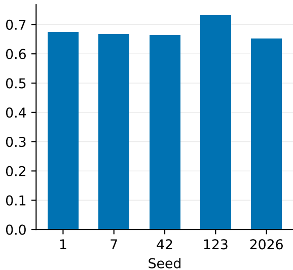
Cv coherence
