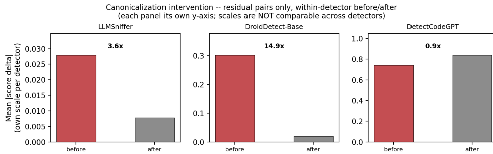
Figure 2: Canonicalization reduction factor, residual pairs only, per detector. Each panel uses its own y -axis; the factors are not cross-comparable, only within a detector’s own scale.
