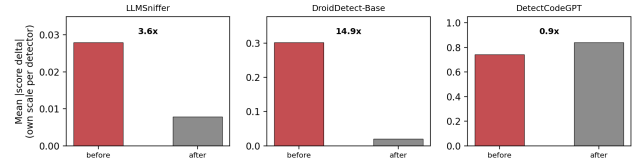
Figure 2: Canonicalization reduction factor, residual pairs only, per detector. Each panel uses its own y-axis; the factors are not cross-comparable, only within a detector’s own scale.
