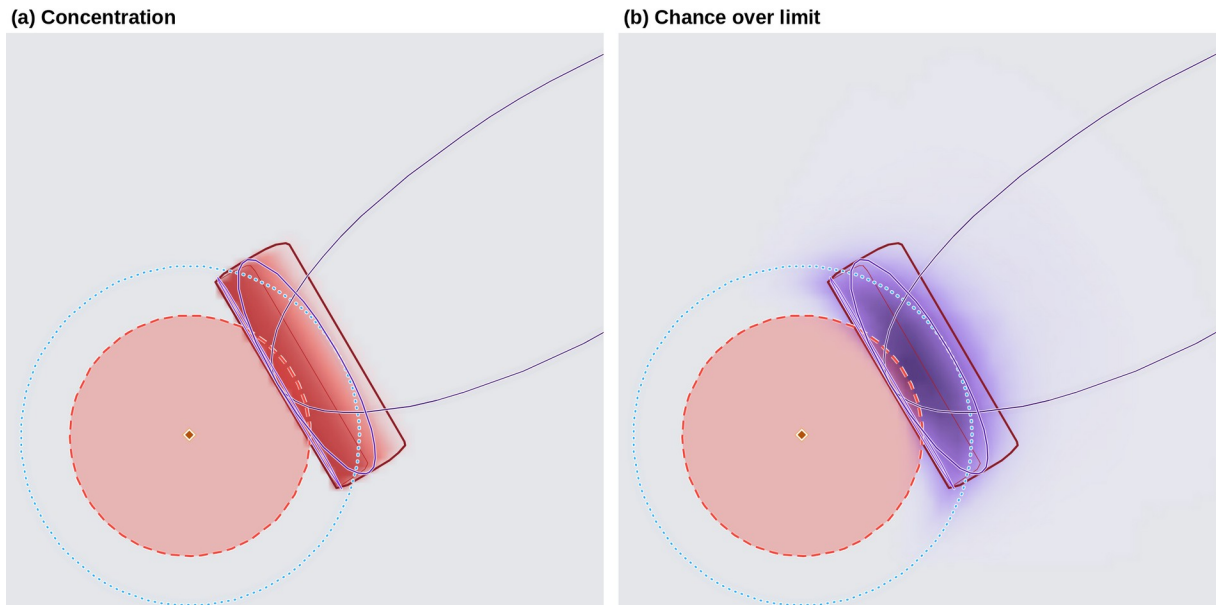
Figure 8.2: The plume at the belt site near Narwapahar (TDS, 20 years; local build, September 2026, drawn without the background map tiles): (a) the concentration field and (b) the chance over the limit, fanned by the measured flow-direction uncertainty. The pink disc is the leach zone, the dotted circle is the monitoring ring and the thin outline is the ML P90 envelope.
