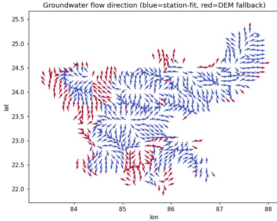
Figure 4.1: The groundwater flow field used by the model: arrows point down-gradient on a 5 km grid; blue cells are fitted from CGWB stations and red cells use the terrain fallback. Data: CGWB levels [3] and GLO-30 DEM [21].
