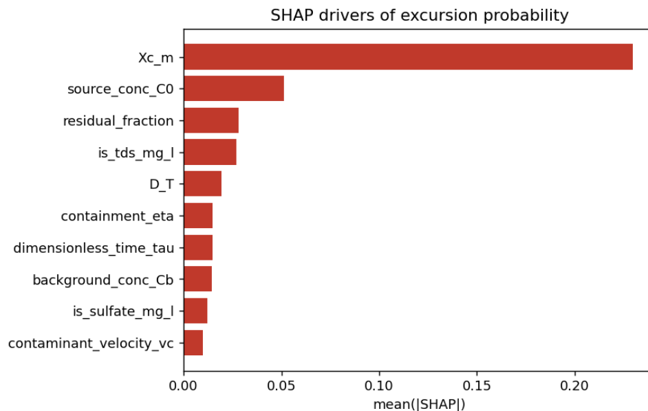
Figure 7.2: SHAP feature importance for the excursion-probability model (version 5): the plume front position calculated by the engine (Xc_m) dominates.
