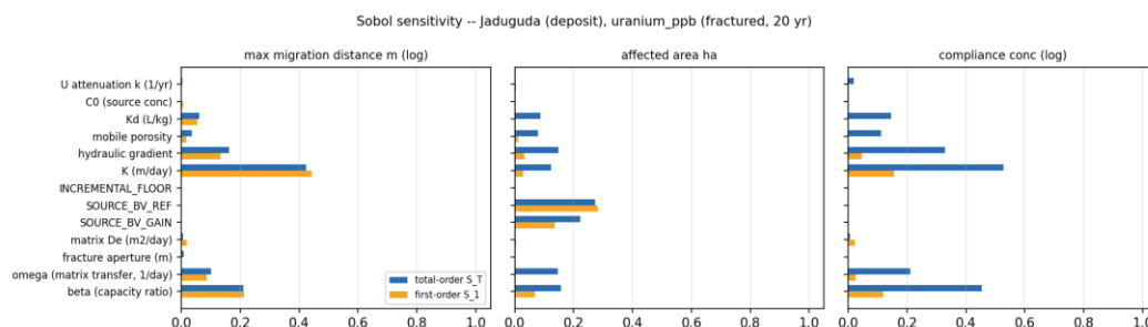
Figure 7.4: Sobol total-order sensitivity indices for uranium at the Jaduguda deposit location, for travel distance, footprint area and ring concentration.
