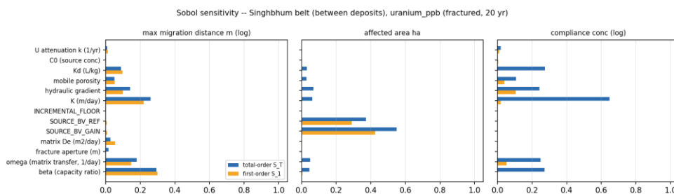
Figure 14.3: Sobol sensitivity indices for uranium at the belt location, where \beta becomes the most important input for travel distance.
