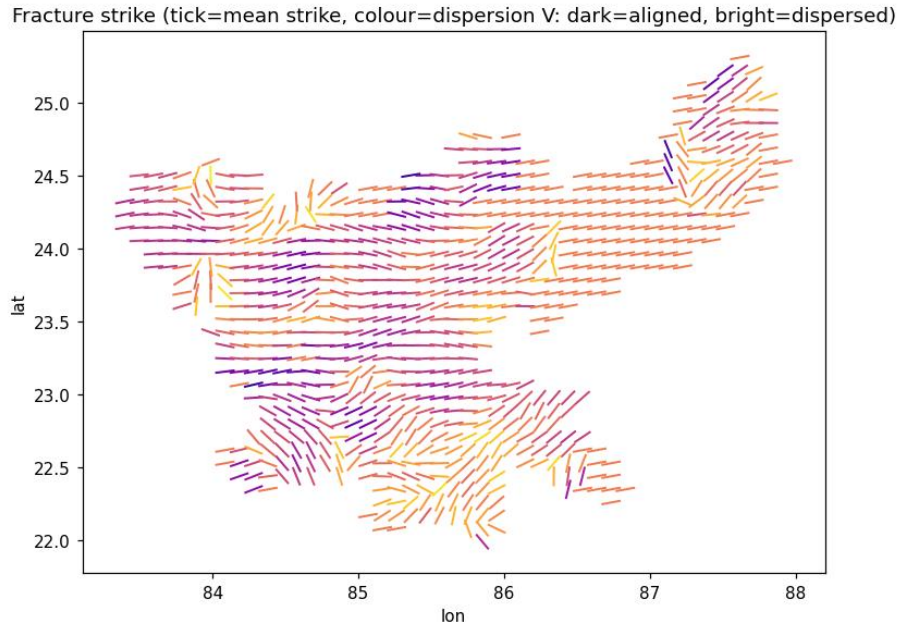
Figure 4.2: The fracture-direction field: each tick shows the average fracture direction in a 5 km cell; the colour shows how scattered the fractures are. Data: GSI–NRSC lineaments [21].
