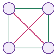
in this drawing two edges cross ...
