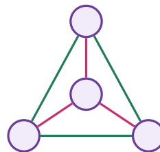
... but the same graph redrawn has no crossings: still planar
