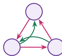
more edges: still an SCC
