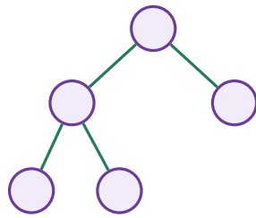
a tree : n = 5 vertices, m = 4 = n - 1 edges
