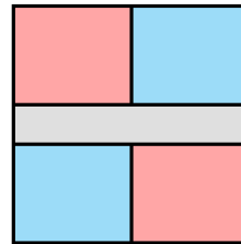
blown up: now blue, blue is not allowed
