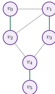
a perfect matching: three pairs
