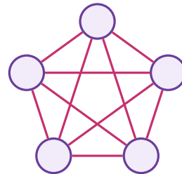
a complete graph: n = 5 , m = \binom{5}{2} = 10 edges
