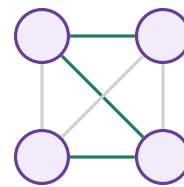
a “Z” shape
