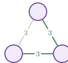
and a third
