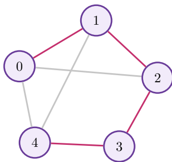
one spanning tree
