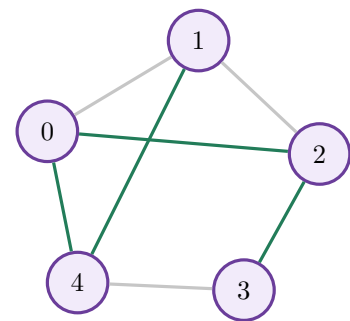
and a third
