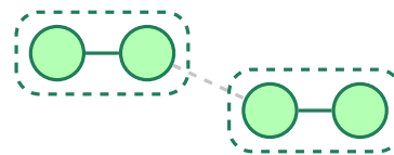
Kruskal: separate pieces get joined together
