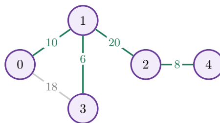
the tree Prim builds: cost 44
