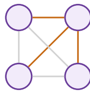
two edges and a diagonal
