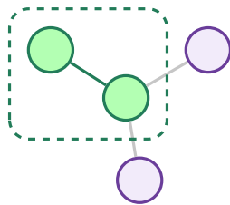
Prim: one tree grows outwards
