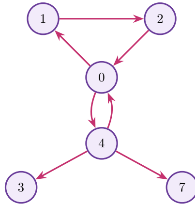
A — paths of length 1
