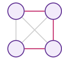
three outside edges
