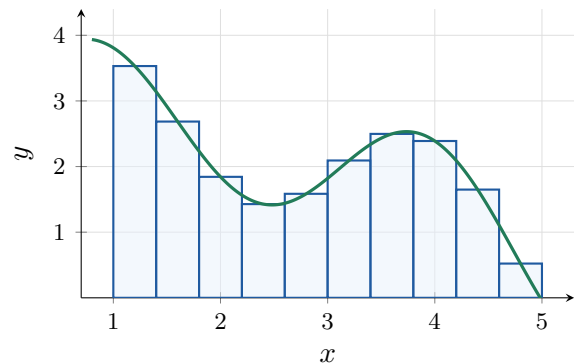
midpoint sum, n = 10
