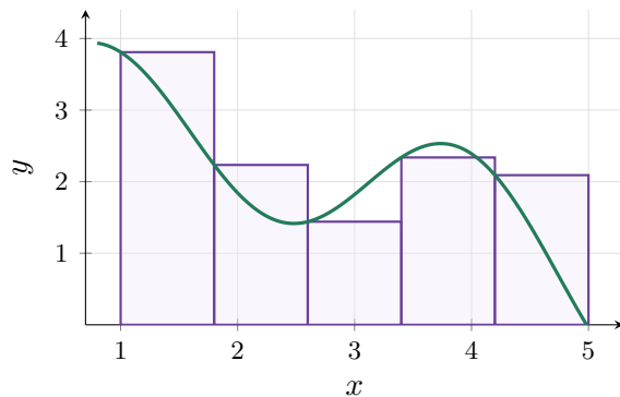
left-hand sum, n = 5
