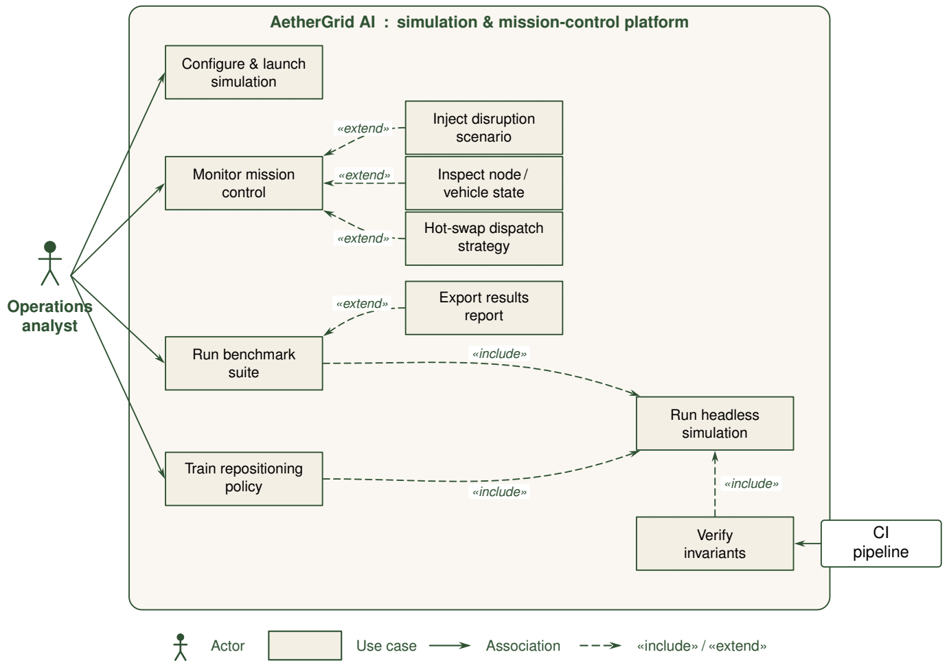
Figure 1: Use Case Diagram. Disruption injection, node telemetry inspection, and strategy hot-swapping extend live monitoring; benchmarking, policy training, and verification include the underlying headless simulation core.
