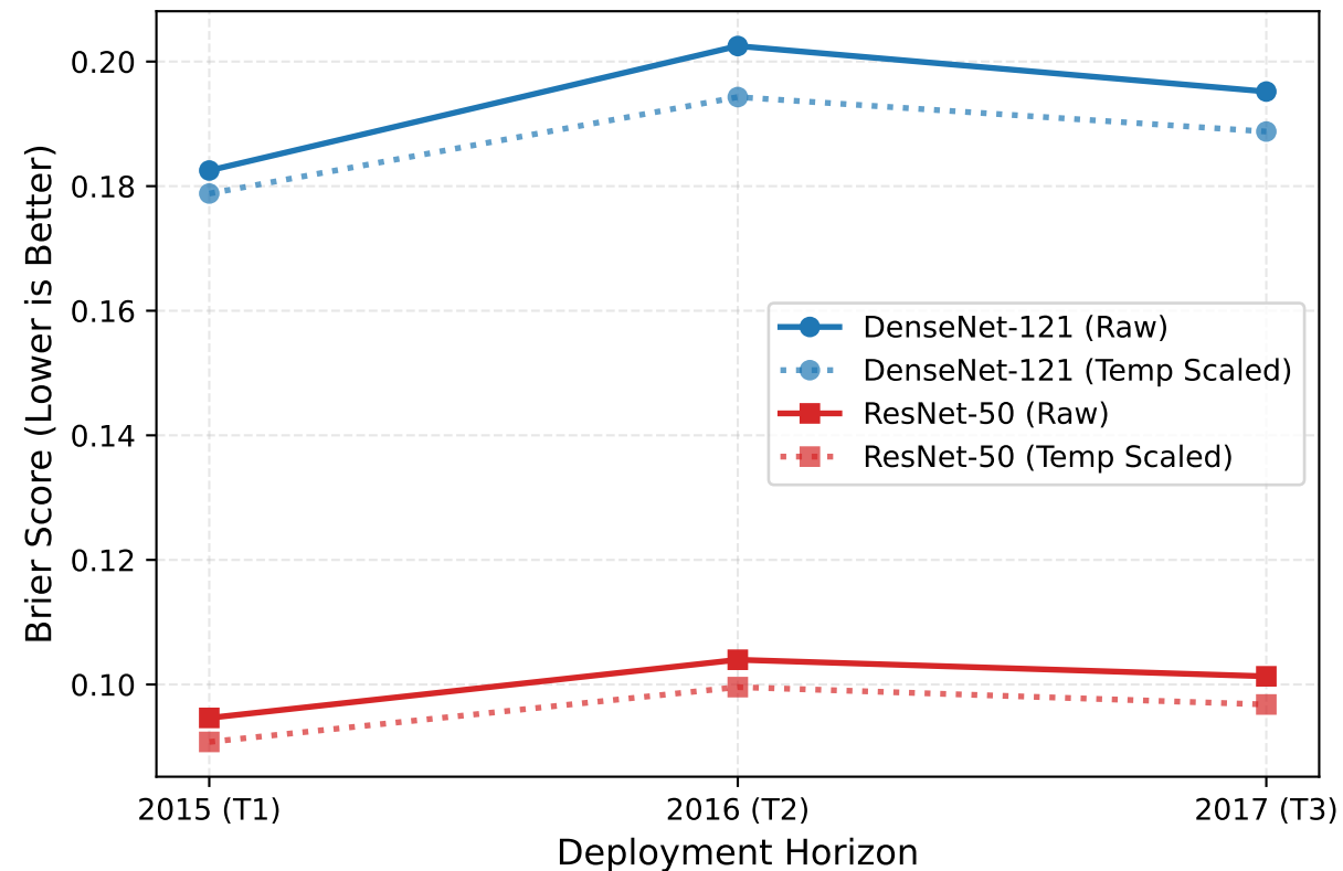
(B) Total Clinical Risk (Brier Score)
