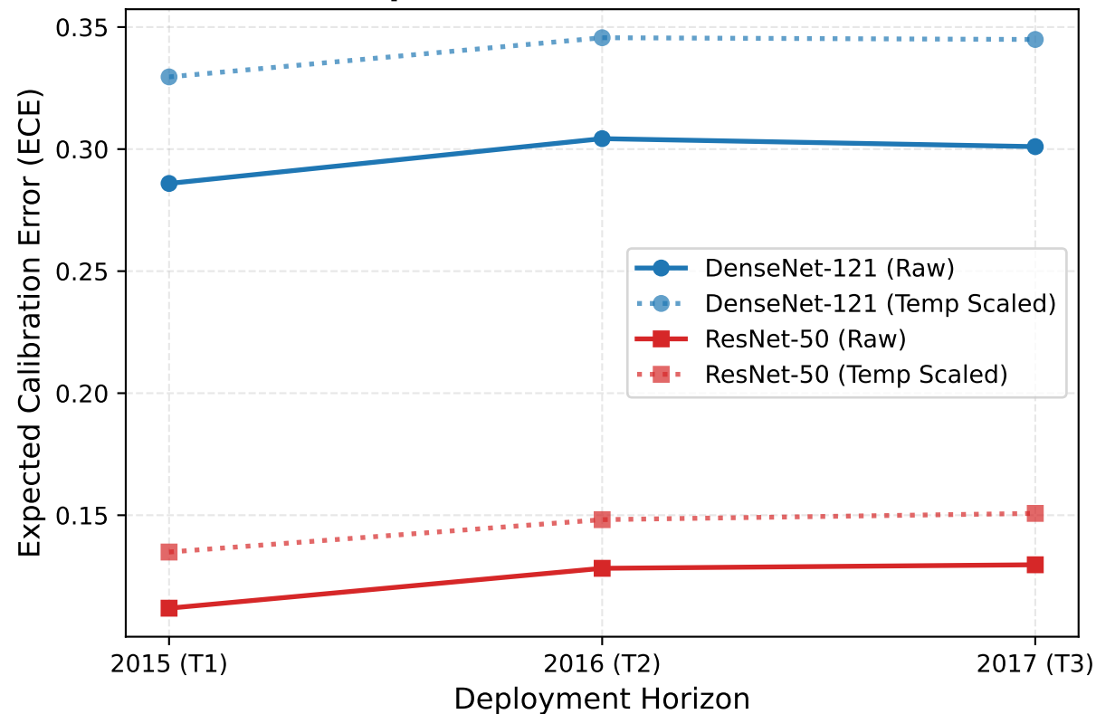
(A) Expected Calibration Error (ECE)
