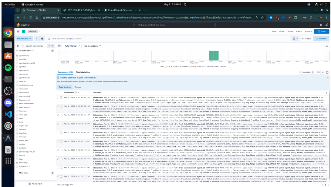
Figure 17: Kibana Discover Tab showing live, structured log streams
