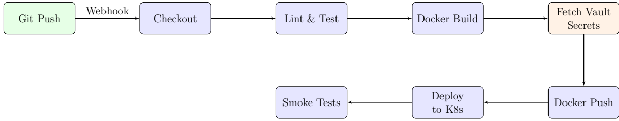
Figure 7: Jenkins CI/CD Pipeline Execution Flow
