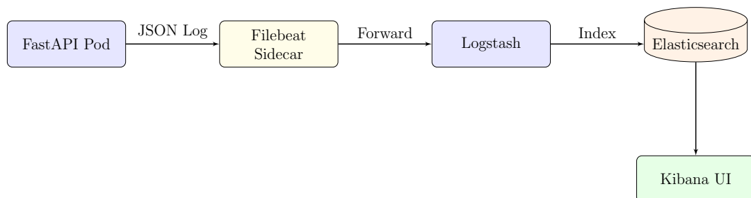
Figure 13: ELK Centralized Logging Architecture
