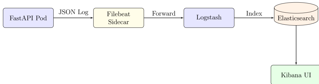
Figure 20: ELK Centralized Logging Architecture
