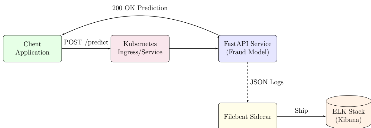
Figure 2: High-Level Request and Processing Flow
