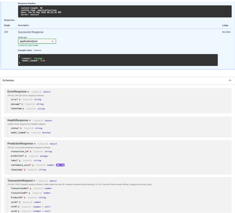
Figure 8: Swagger UI showing detailed TransactionRequest schema fields
