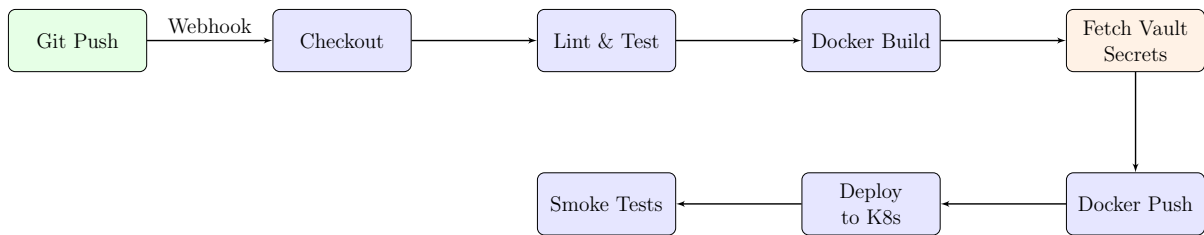
Figure 13: Jenkins CI/CD Pipeline Execution Flow
