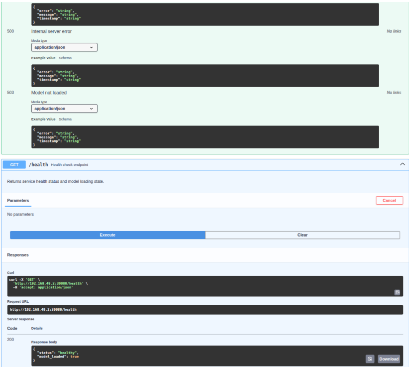
Figure 7: Swagger UI showing API request and response schemas
