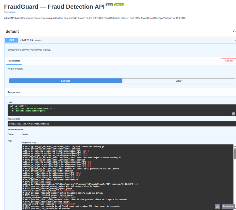
Figure 4: Swagger UI showing Prometheus metrics exposed at the /metrics endpoint
