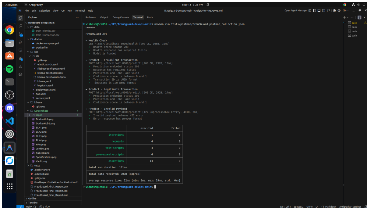
Figure 15: Newman Automated Smoke Tests executing 14 passing assertions against the live Kubernetes API
