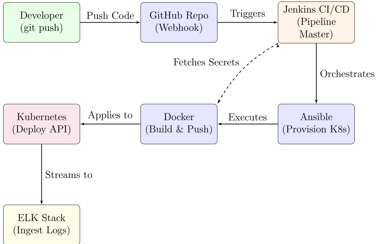
Figure 1: Global End-to-End Execution Sequence Diagram
