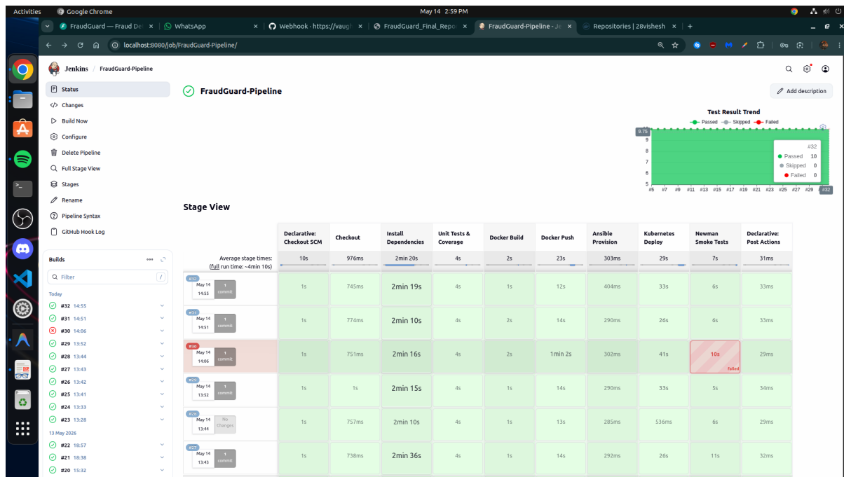
Figure 14: Jenkins Dashboard demonstrating successful pipeline execution across all stages
