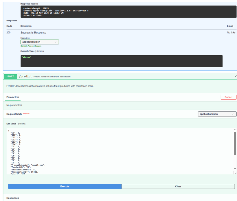
Figure 5: Swagger UI showing successful execution of the /predict endpoint with a legitimate transaction response
