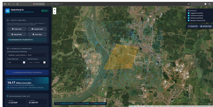
Fig. 3. Web GIS analytical run for the primary village benchmark parcel, showing optimal drainage convergence at elevation 288.7 m with 14.17 Million Litres (14, 173 m 3 ) estimated runoff collection.
