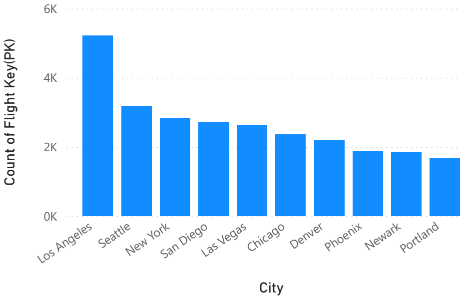
Count of Flight Key(PK) by City
