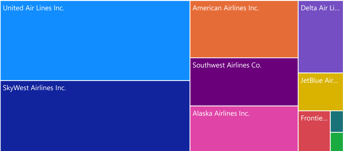
Sum of Total Delay by Airline Name
