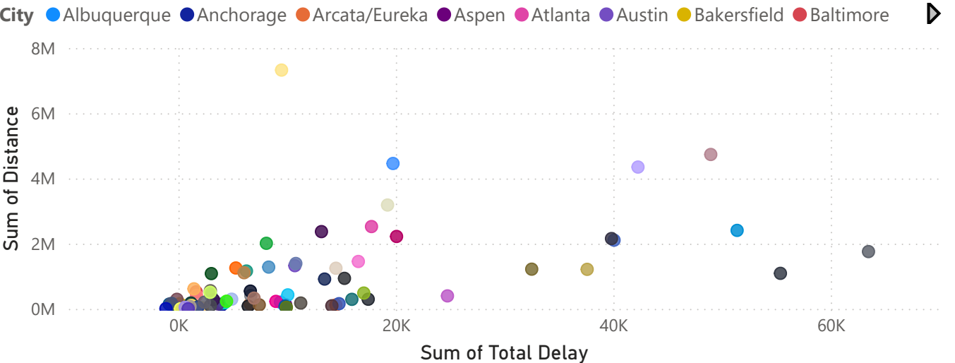
Sum of Total Delay and Sum of Distance by City and City
