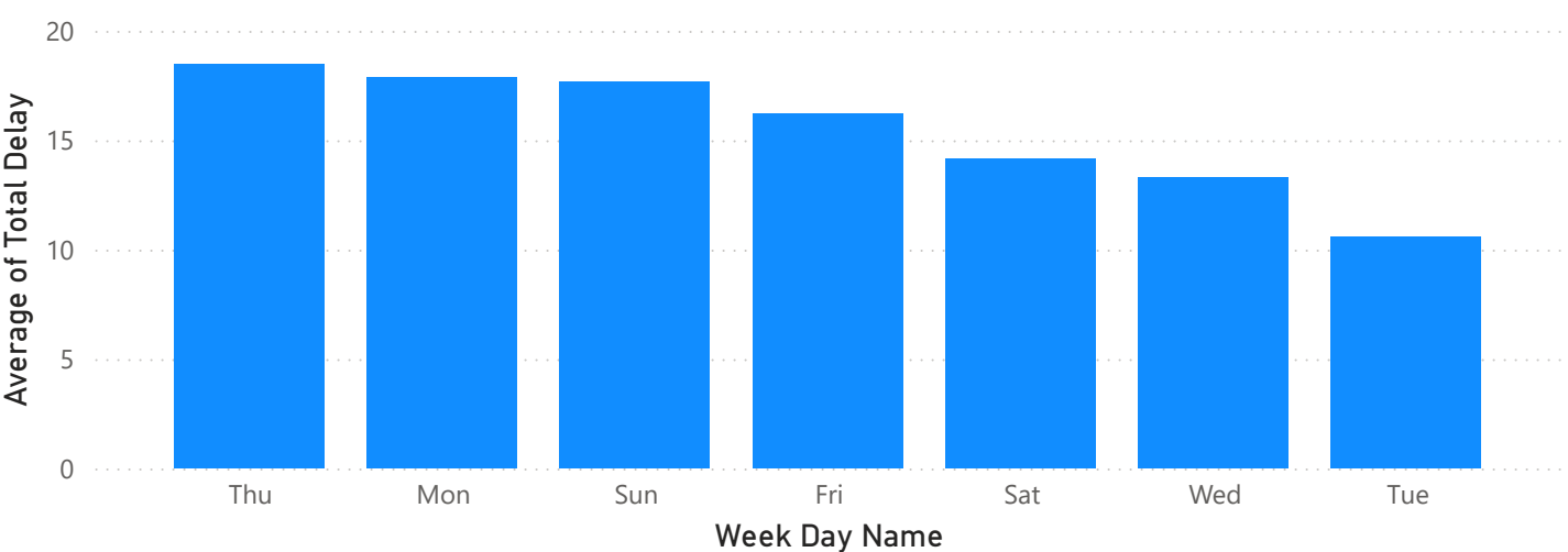
Average of Total Delay by Week Day Name
