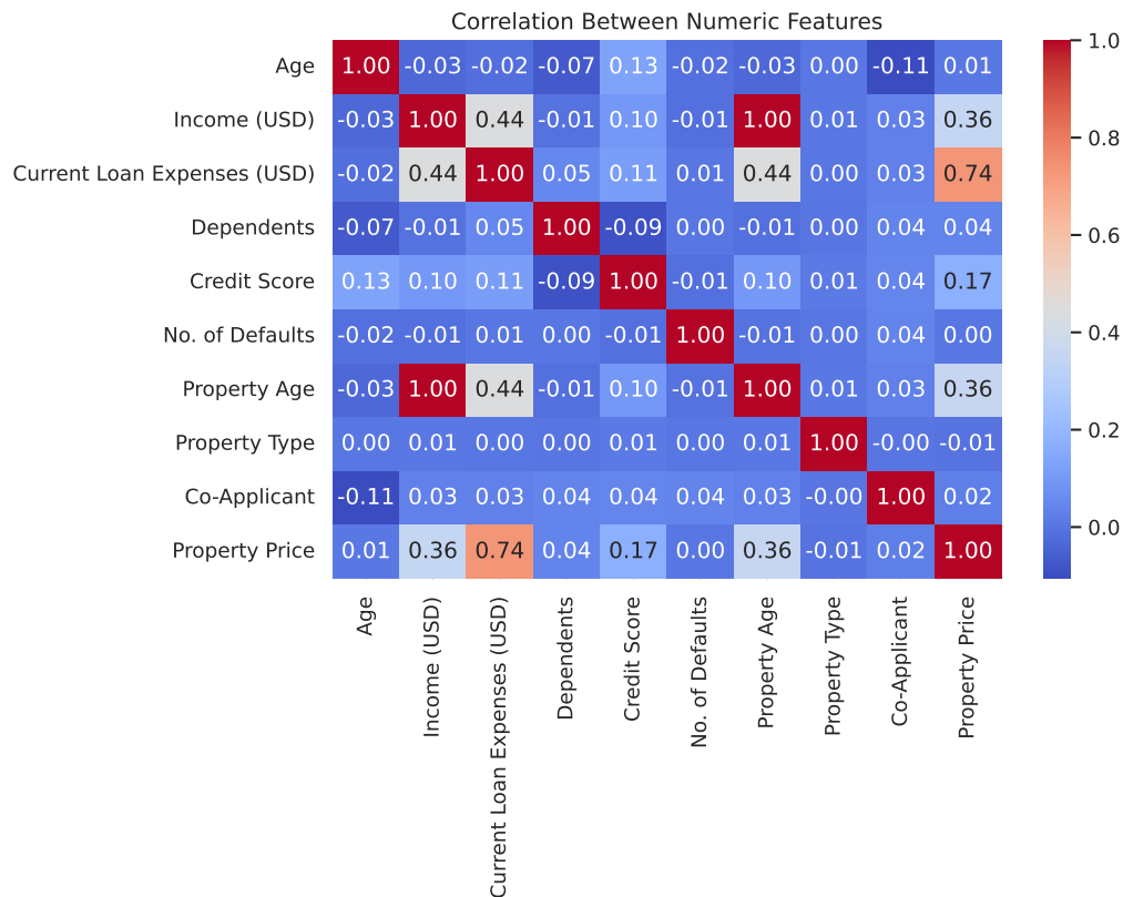
Figure 4: Pearson correlation between numeric features
