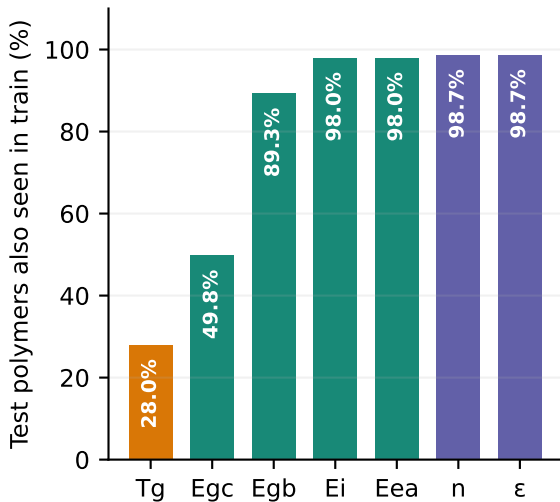
Cross-property support differs by target
