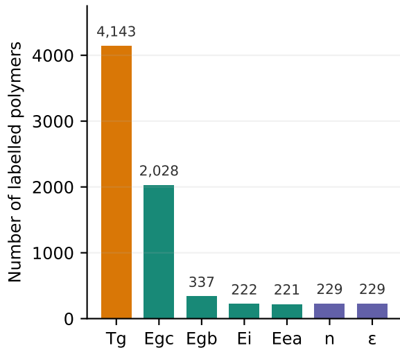
Training labels are highly uneven
