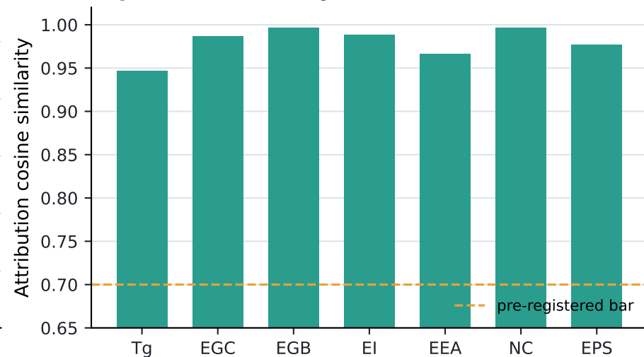
Explanation stability
