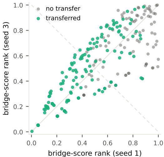
Spearman \rho = +0.84
