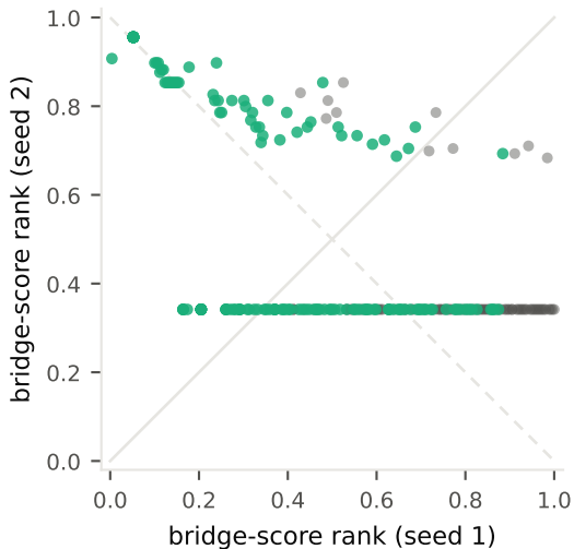
Spearman \rho = -0.59
