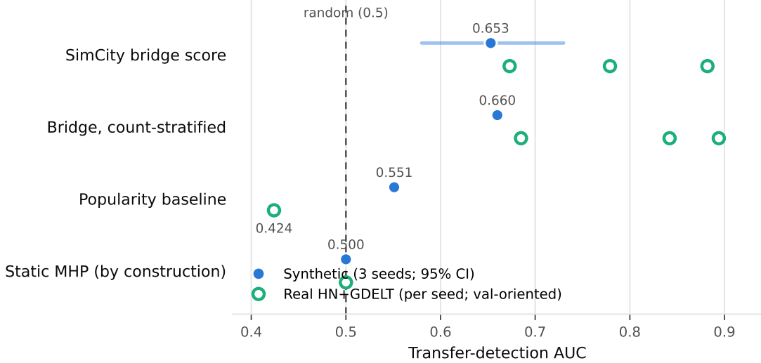
Figure 1: Narrative transfer detection AUC . Synthetic benchmark (filled blue: three-seed mean with bootstrap 95% CI) vs. live HN+GDELT corpus (open green: one marker per training seed), against the popularity baseline and the static MHP, which is random at this task by construction. On the controlled benchmark the bridge score is stable and significantly above random and the popularity baseline. Real-corpus values are per-seed and validation-oriented : the likelihood does not identify the head’s sign (seeds agree up to mirror image, \rho = 0.96 ), so each head’s orientation is fixed on the validation split only — no test leakage — yielding 0.882/0.673/0.779, every seed individually significant (section 8.3(4)). The popularity baseline is anti-predictive on the real corpus.
