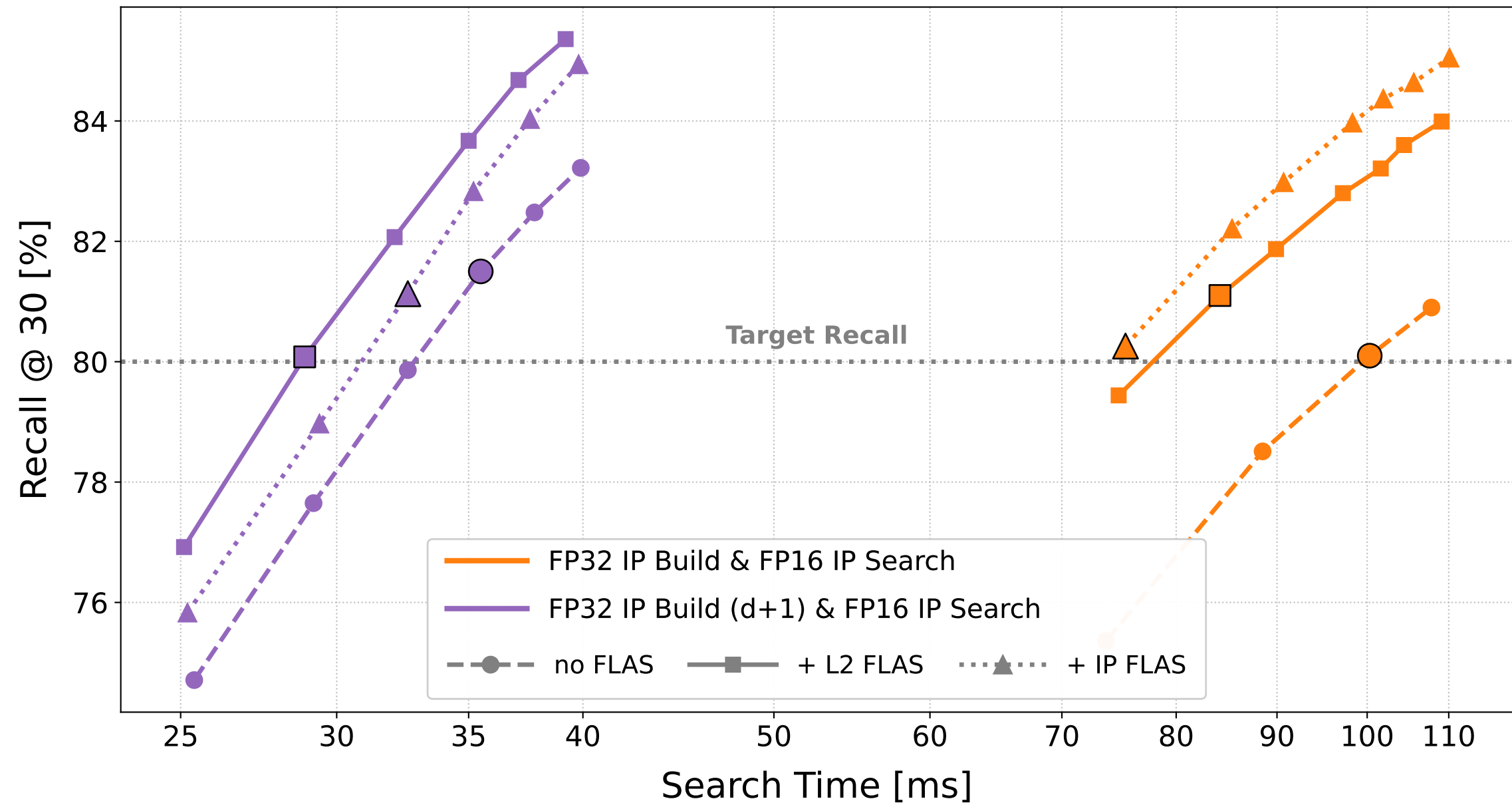
Task 2 Benchmark — Recall @ 30 vs Search Time
