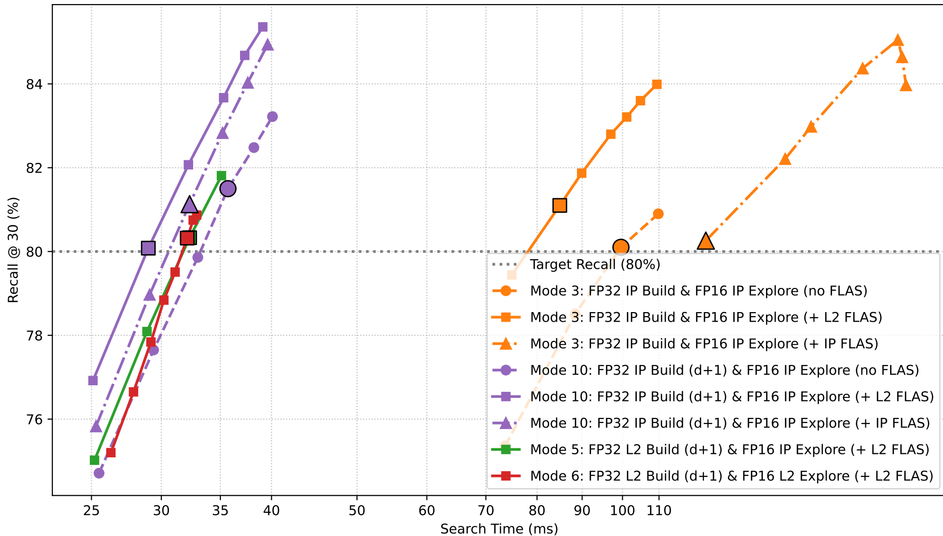
Task 2 Benchmark — Recall @ 30 vs Search Time
