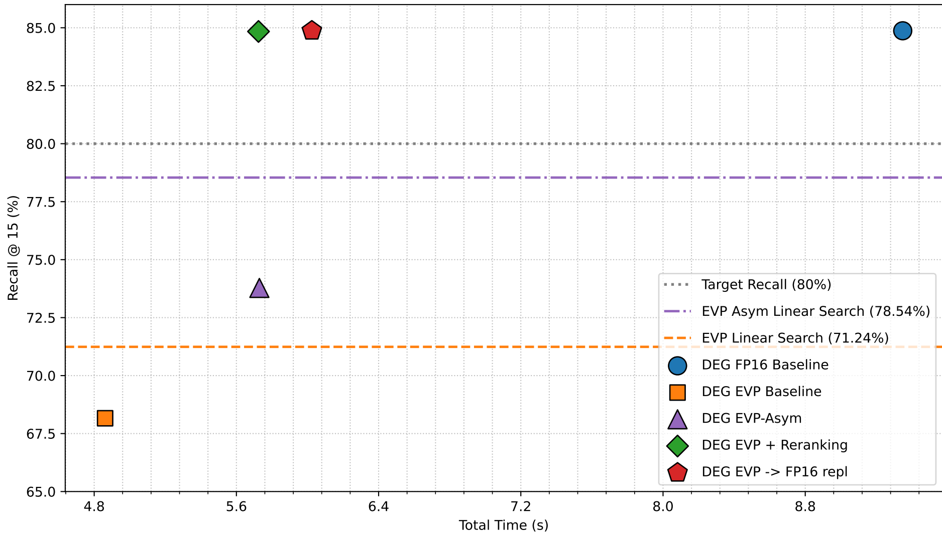
Task 1 Small Benchmark — Recall vs Total Time
