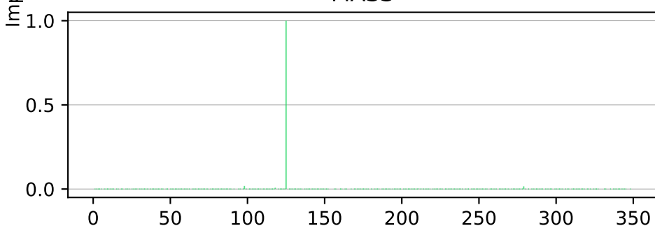
SASA
