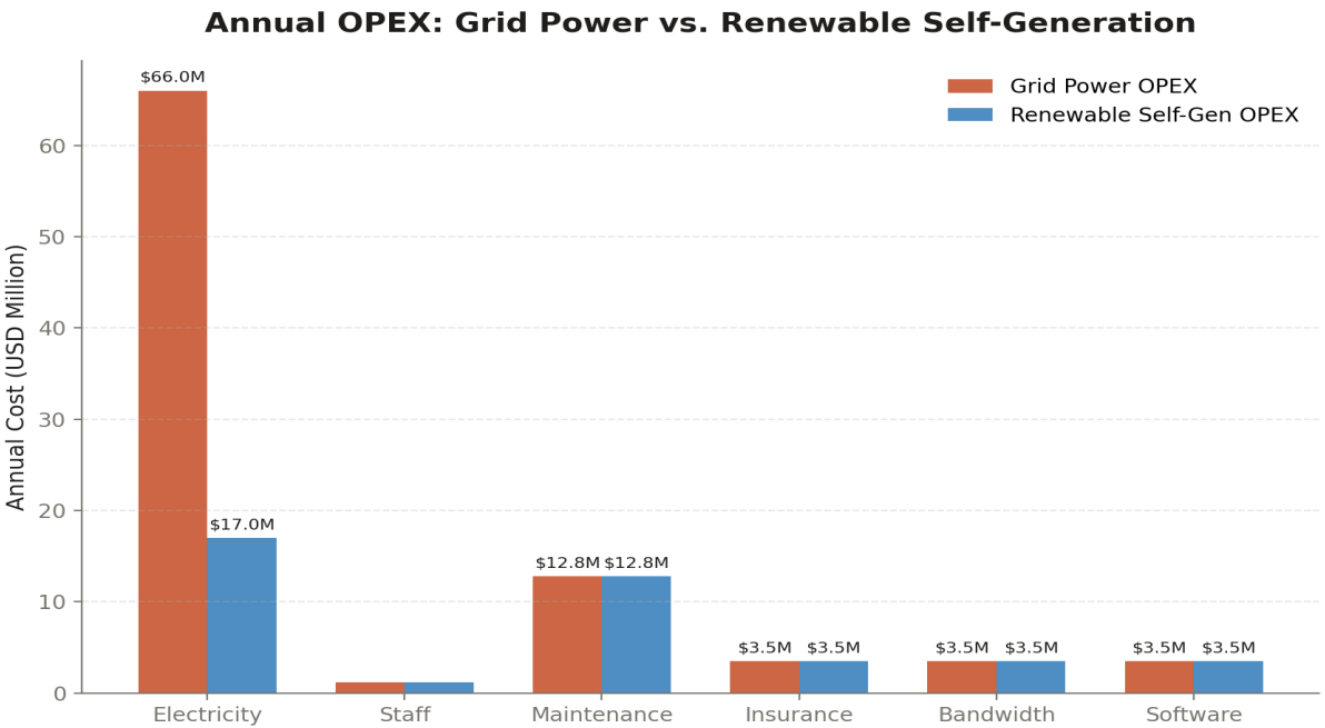
Figure 7: Annual OPEX - Grid Power vs. Renewable Self-Generation
