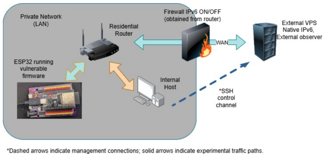
Figure 3.1: Overview of the Testbed Architecture
