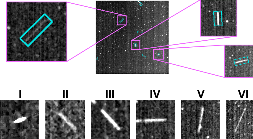
Morphological groups
