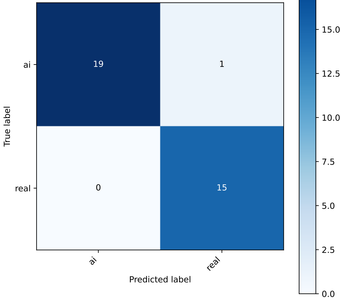
Confusion Matrix
