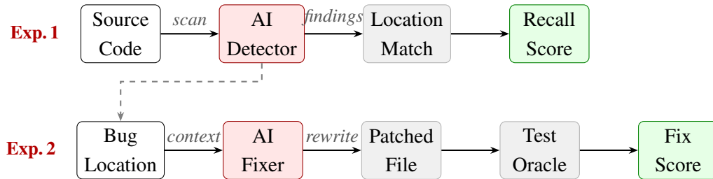
Figure 1: End-to-end pipeline architecture. Experiment 1 runs the detector and scores recall. Experiment 2 feeds the detector’s findings to the fixer, then runs the oracle to produce the fix verdict. The dashed arrow shows findings flowing from detection into the fix prompt.
