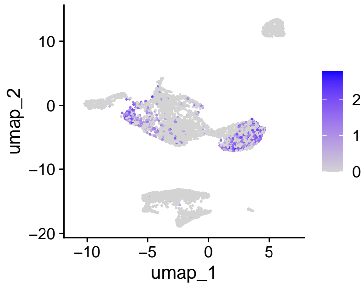
CD8B
