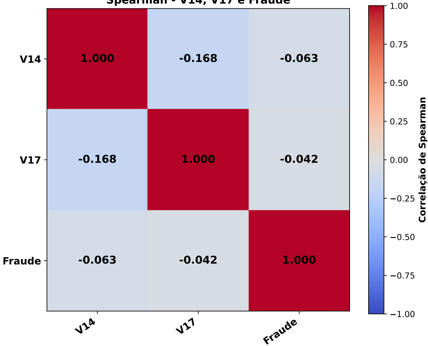
Spearman - V14, V17 e Fraude
