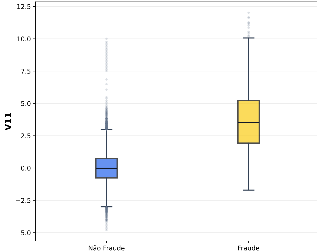
Boxplot - V11
