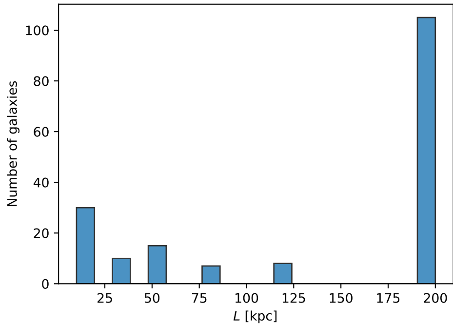
(a) Distribution of L
