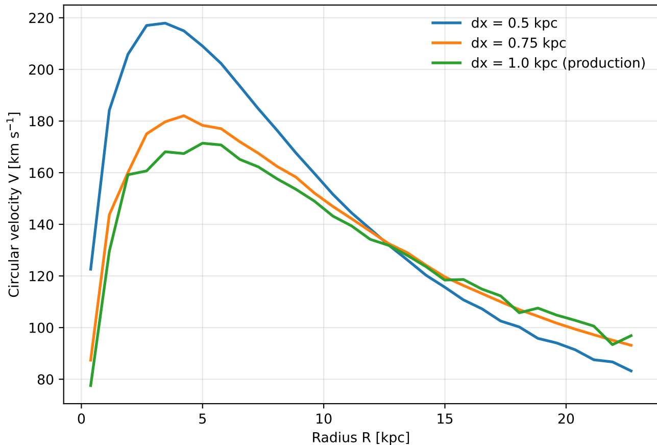
Resolution Invariance Test — NGC 4559
