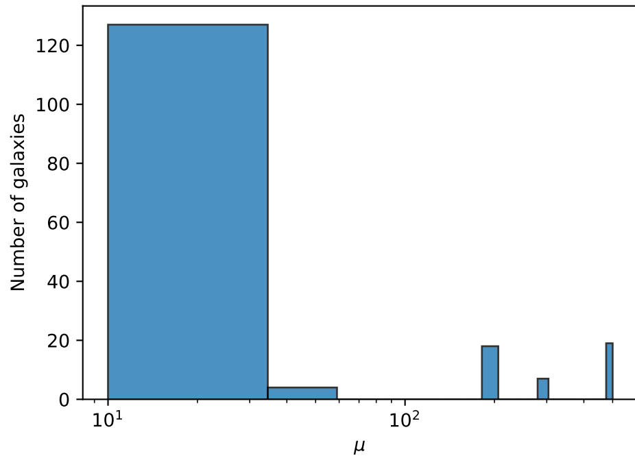
(b) Distribution of \mu
