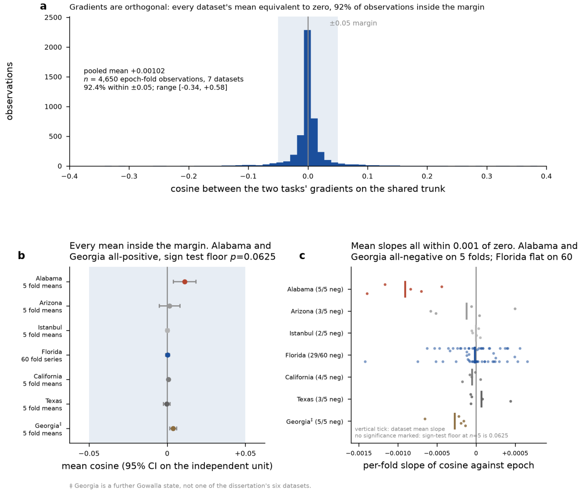
Figure 8 – The two tasks' gradients on the shared trunk are orthogonal, on seven datasets: the six of Chapter 5 and Georgia, marked † because the dissertation does not otherwise use it. The shaded band is the equivalence margin of \pm 0.05 ; every mean falls inside it. Panels: (a) the pooled distribution of all 4,650 epoch-level cosines, (b) each dataset's mean with its 95 percent interval on the independent unit, (c) one point per fold for the slope of the cosine against the epoch, with a tick at each dataset's mean slope. No significance is marked anywhere in the figure.
