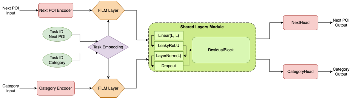
Figure 1 – The proposed Multi-Task Learning (MTL) architecture. Task-specific encoders process inputs for POI Category Classification and Next-POI Prediction. Feature-wise Linear Modulation (FiLM) layers adapt these features using learnable task embeddings. The modulated representations are then processed by a shared path of residual blocks. Finally, dedicated task-specific heads generate the respective outputs.
