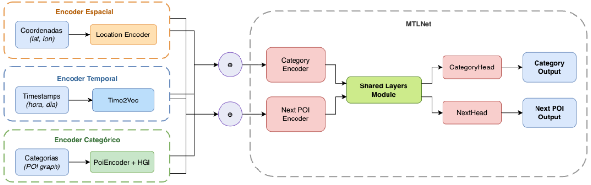
Figure 2 – Architecture based on MTLNet (39). The spatial, temporal, and categorical encoders are trained in a decoupled manner and generate their respective embeddings , which are integrated as input to the model. The integrated input is processed by the model’s shared layers ( Shared Layers Module ) and by the task-specific layers, producing the Category Output and Next POI Output .
