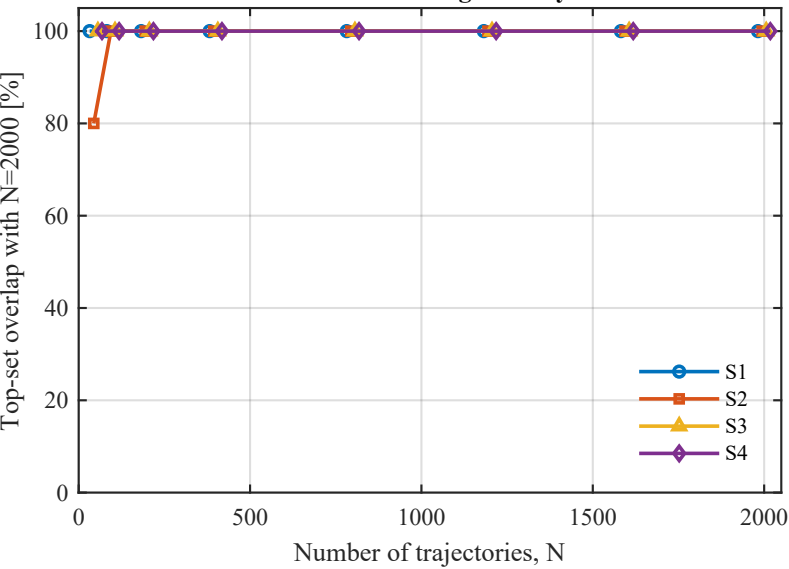
Branch-ranking stability
