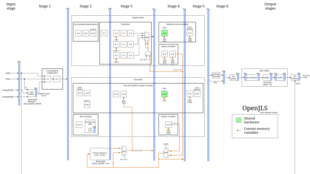
Figure 1: Encoder pipeline architecture.
