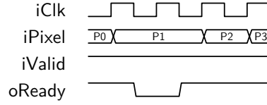
Figure 2: Pixel-input handshake.
