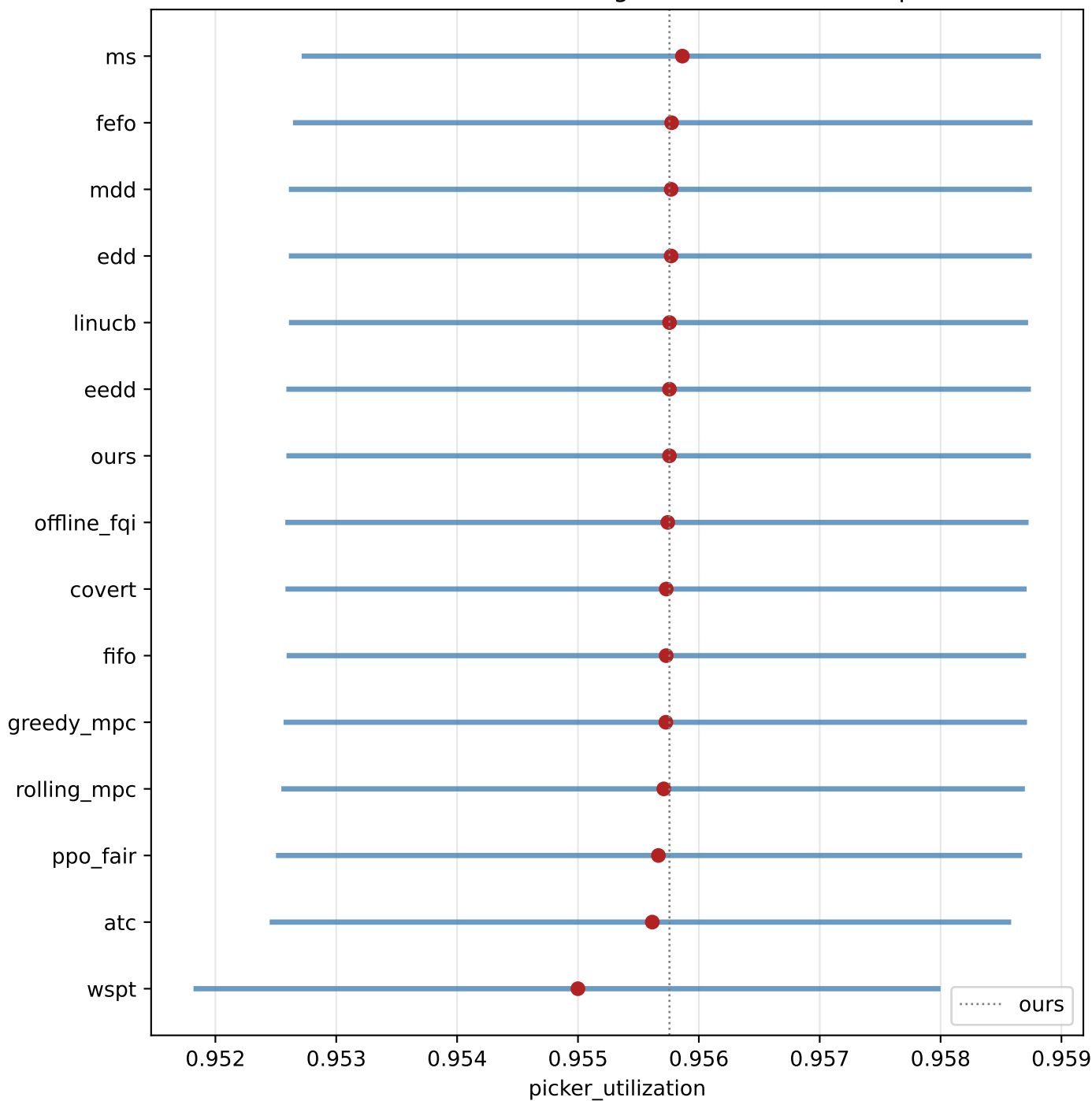
E2 — picker_utilization (scenario=default) 50 test shifts · 250 training shifts · 95% bootstrap CI
