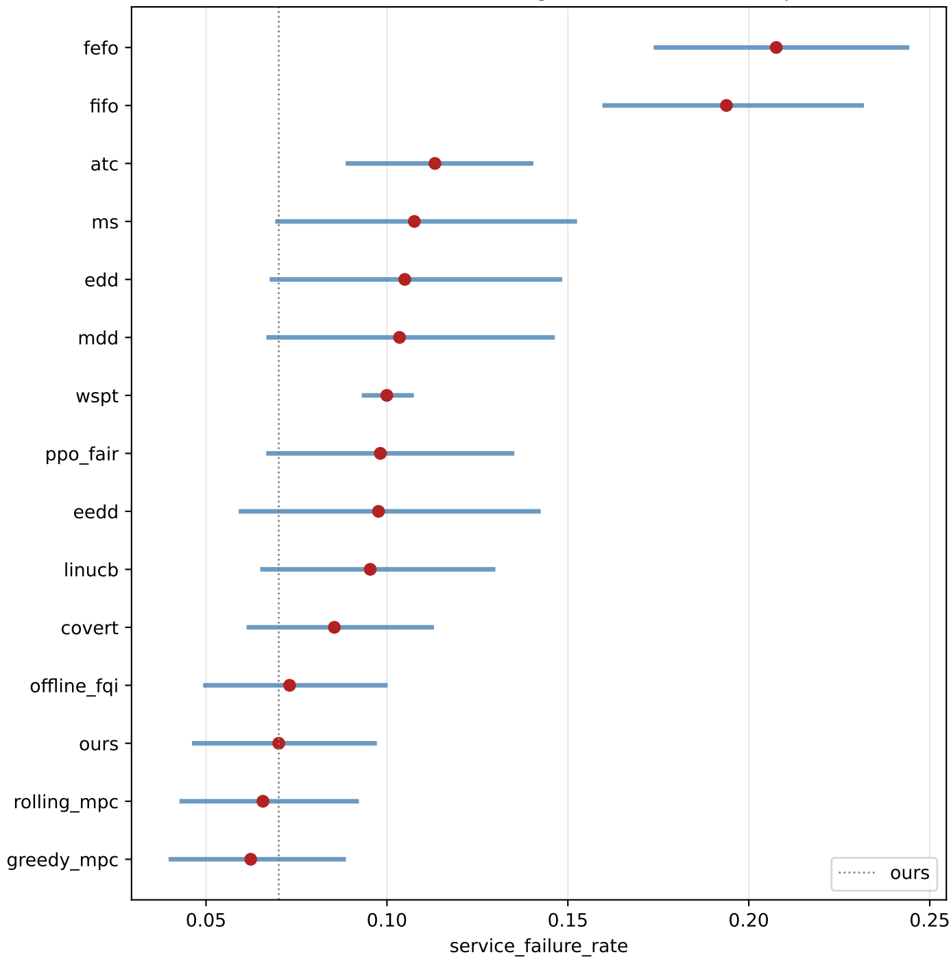
E2 — service_failure_rate (scenario=default) 50 test shifts · 250 training shifts · 95% bootstrap CI
