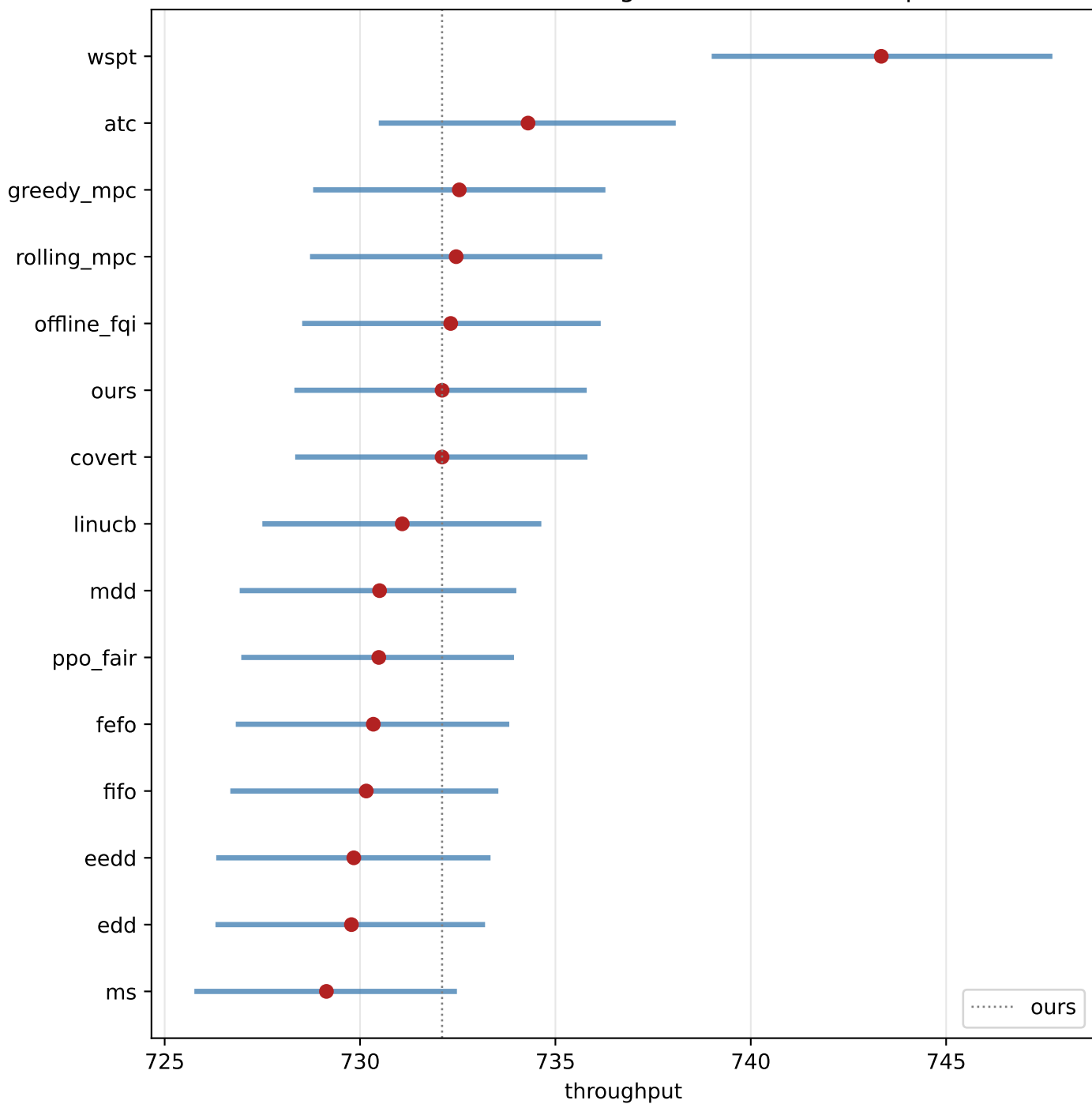
E2 — throughput (scenario=default) 50 test shifts · 250 training shifts · 95% bootstrap CI
