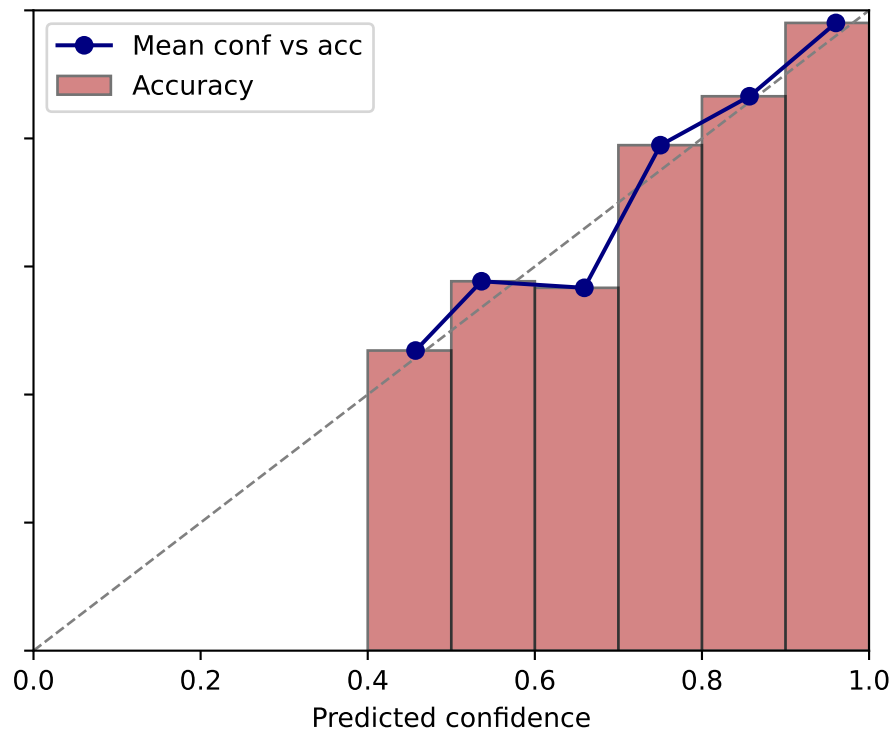
Post-calibration (isotonic) ECE = 0.0198
