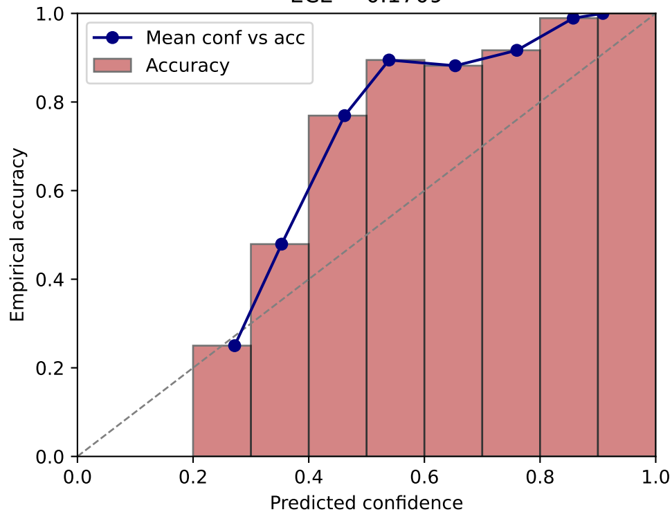
Pre-calibration ECE = 0.1709
