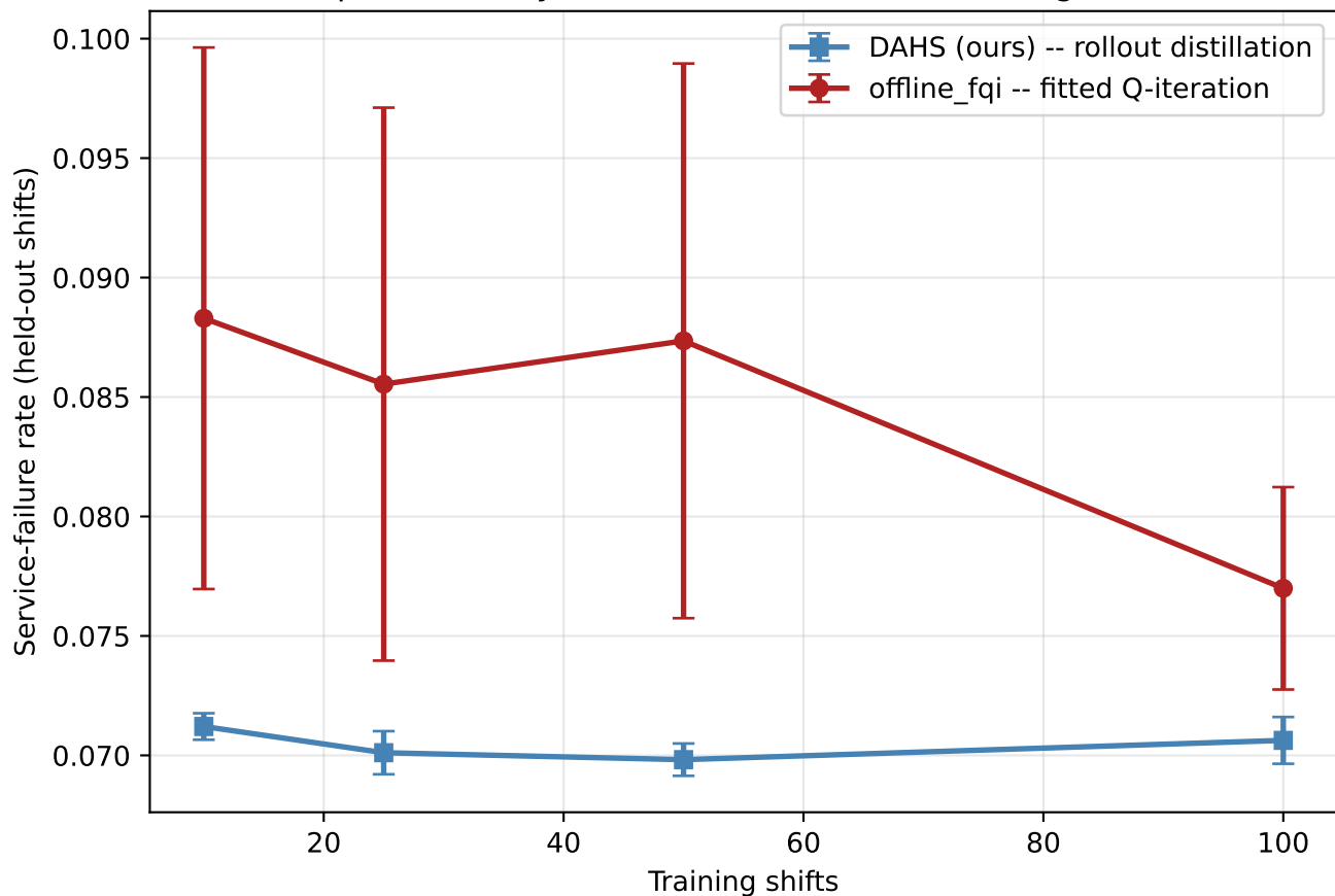
Sample efficiency: DAHS vs offline value-learning baseline
