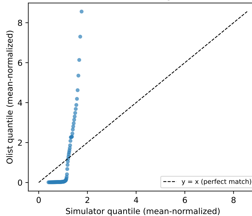
Processing time KS D=0.685 W=1.101
