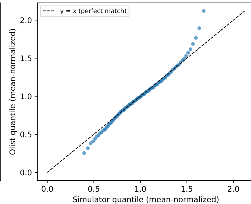
SLA / due-date window KS D=0.039 W=0.036
