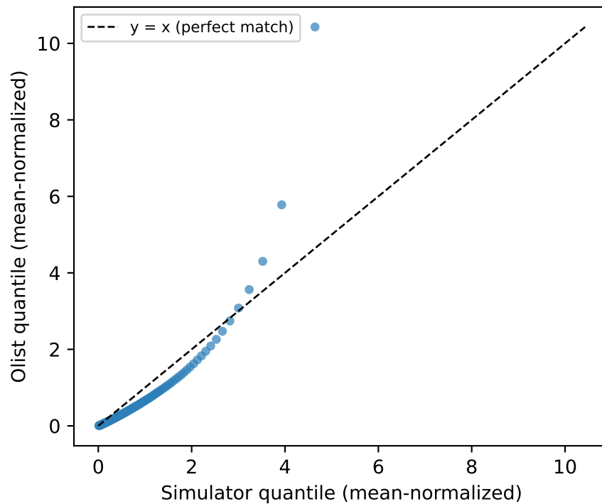
Inter-arrival time KS D=0.153 W=0.443
