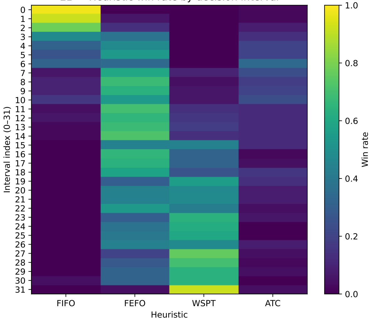
E1 — Heuristic win rate by decision interval
