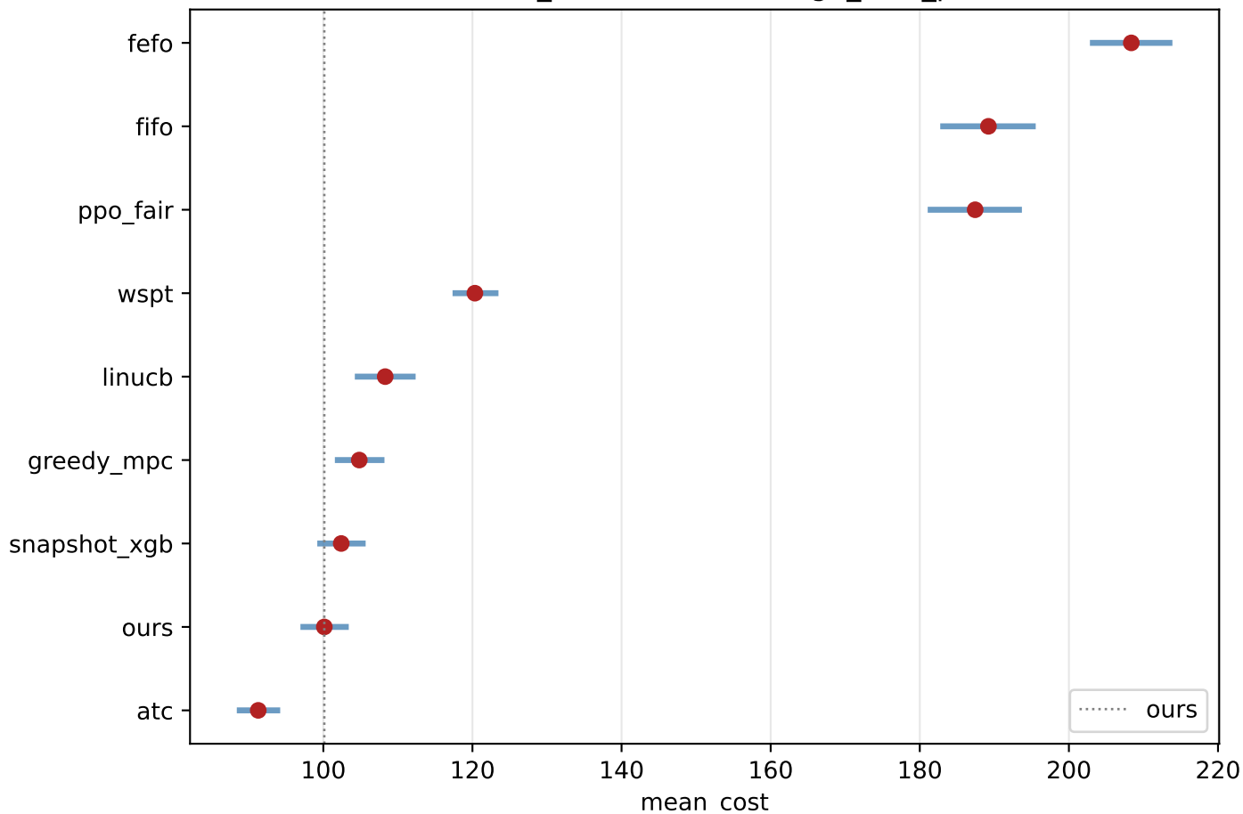
E2 — mean_cost (scenario=high_load_perish)
